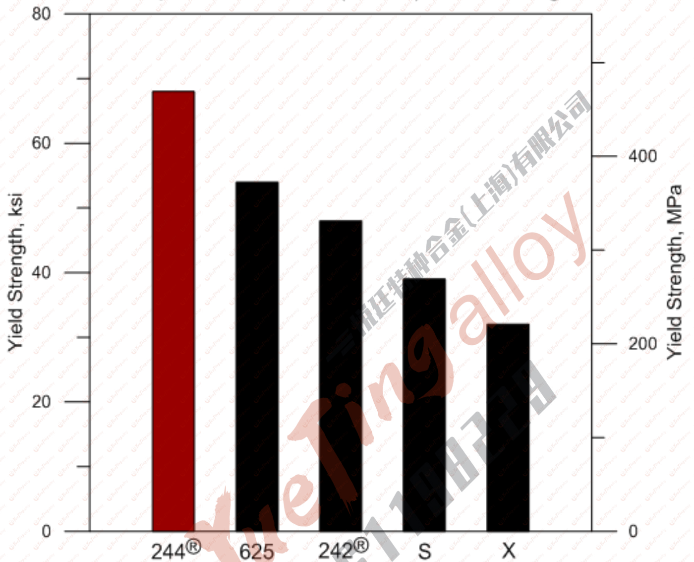
Comparative 1400°F (760°C) Yield Strength
